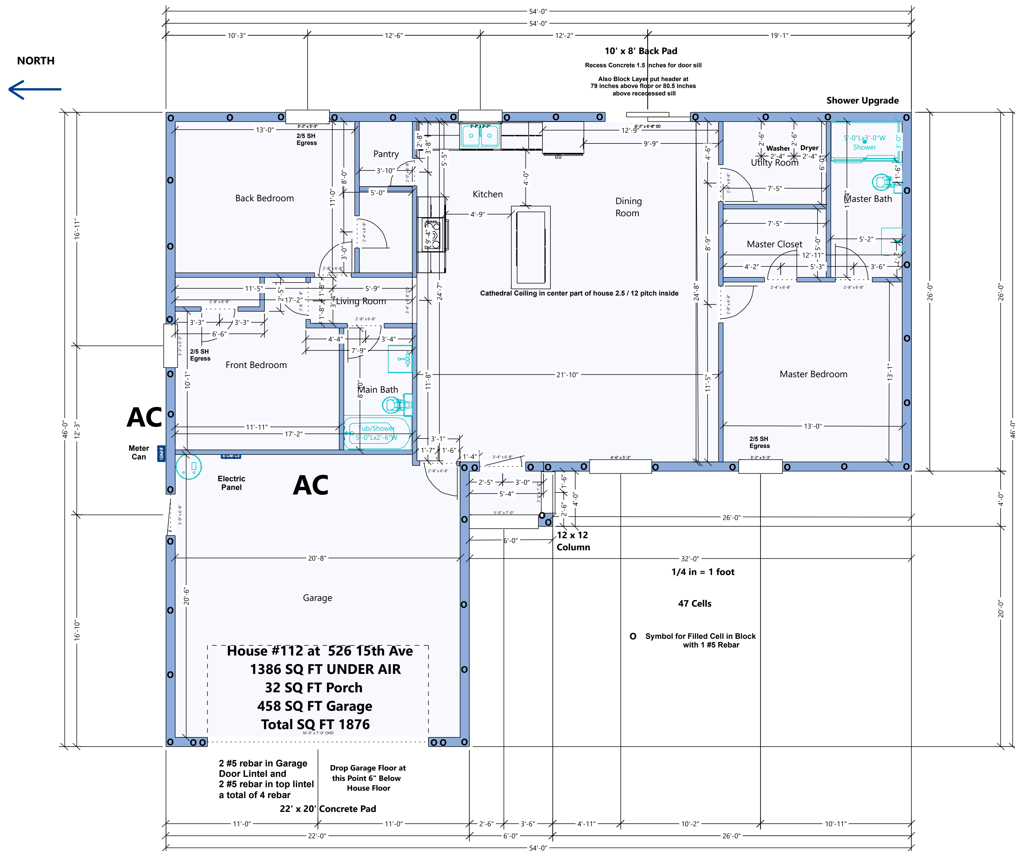
Model AC1386LH FP32 GA458
